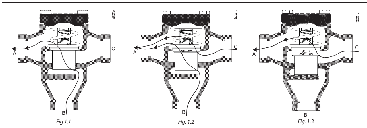
Figure 1: Mixing operation
